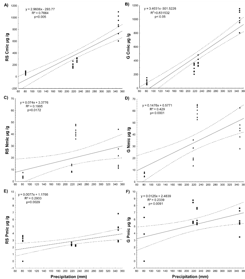
Figure 1 Simple linear regressions between annual accumulated precipitation before the sampling date for four years and nutrients immobilized by microbial biomass for RS soil and G soil. The dotted line represents the standard deviation at 0.95.
