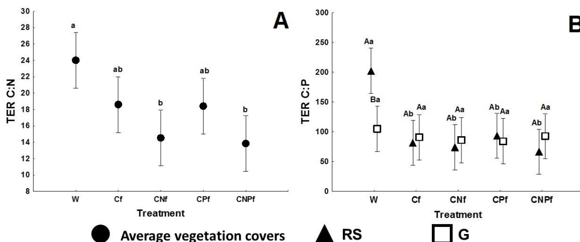
Figure 7. Means and standard errors of: Threshold elemental ratio A) TERC:N, B) TERC:P; under five fertilization treatments in rosetophyllous scrub soil (RS) and the grassland soil (G) of the Cuatro Ciénegas Basin, Coahuila, Mexico. Different uppercase letters (A and B) indicate significantly different means ( P < 0.05 ) between vegetation cover (RS and G) within the same treatment; whereas different lowercase letters vertically indicate significantly different means ( P < 0.05 ) among fertilization treatments within the same vegetation. W: control, Cf: carbon fertilization, CNf: carbon and organic N fertilization, CPf: carbon and organic phosphorus fertilization, and CNPf: carbon, organic N and organic P fertilization.
