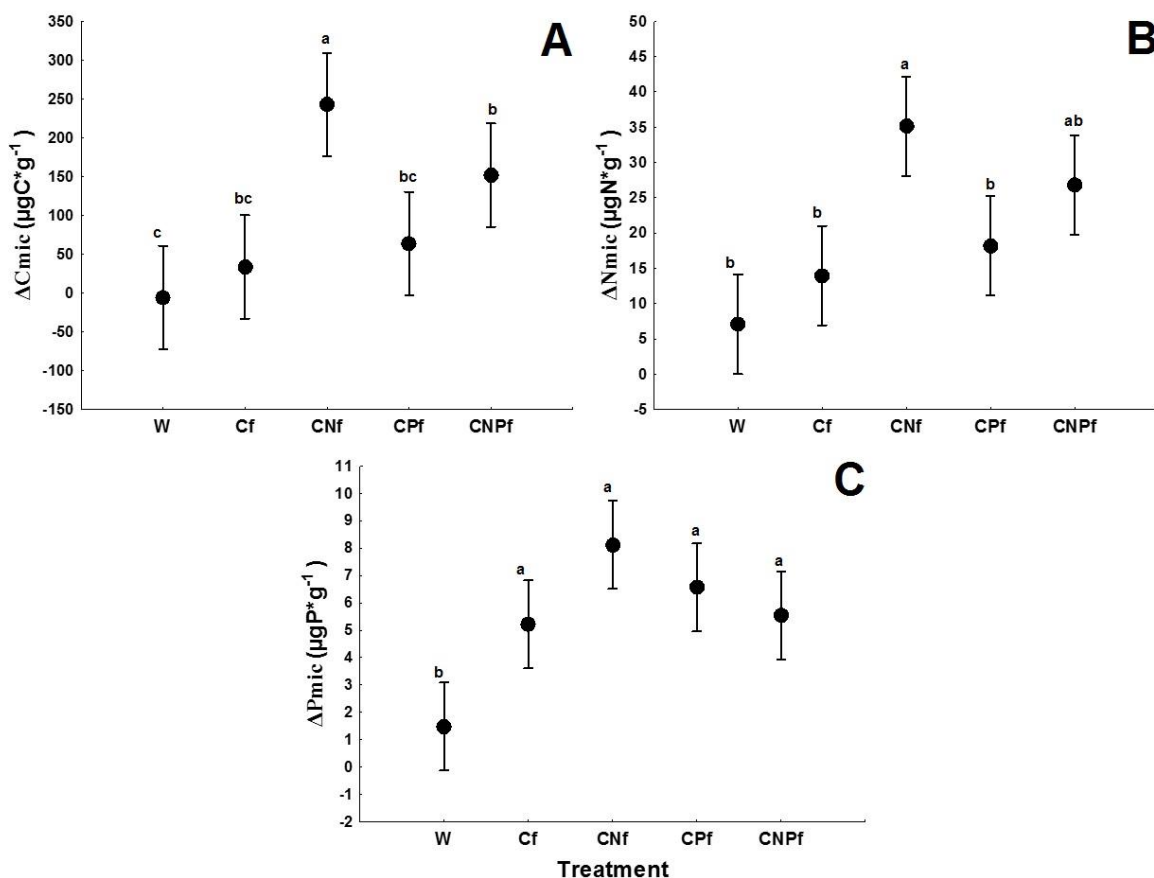
Figure 6. Means and standard errors of potential nutrient immobilization within microbial biomass (A: carbon, B: nitrogen and C: phosphorus) under five treatments in rosetophyllous scrub soil (RS) and the grassland soil (G) of the Cuatro Ciénegas Basin, Coahuila, Mexico. Different lower-case letters indicate significant differences between treatments ( P < 0.05 ). W: control, Cf: carbon fertilization, CNf: carbon and organic N fertilization, CPf: carbon and organic phosphorus fertilization, and CNPf: carbon, organic N and organic P fertilization.
