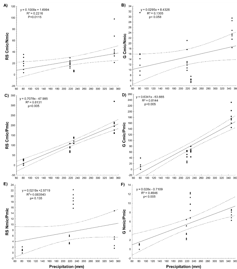
Figure 2 Simple linear regressions between the annual accumulated precipitation before the sampling date for four years and ratios of nutrients immobilized by microbial biomass for RS soil and G soil.
